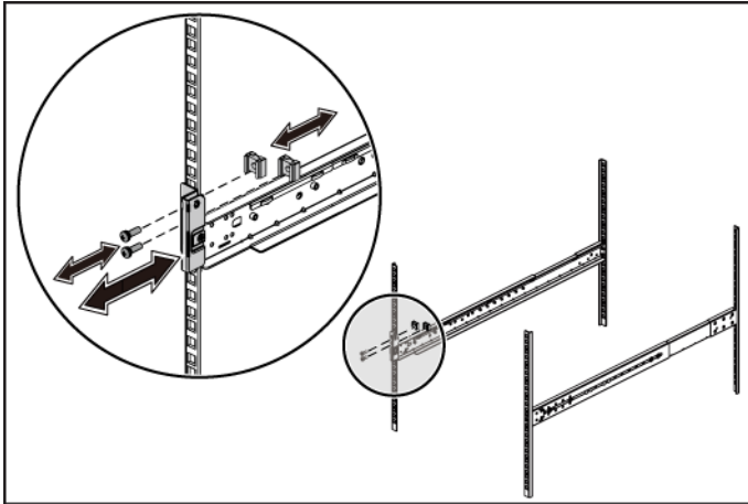
Figure 2. Installing the Chassis Stabilizer Shipping Brackets
