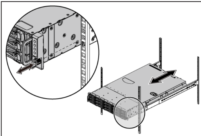
Figure 3. Installing the Chassis onto the Rack.
